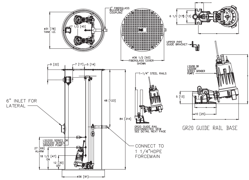
DUPLUX GRINDER PUMP STATION SCALE: NTS
