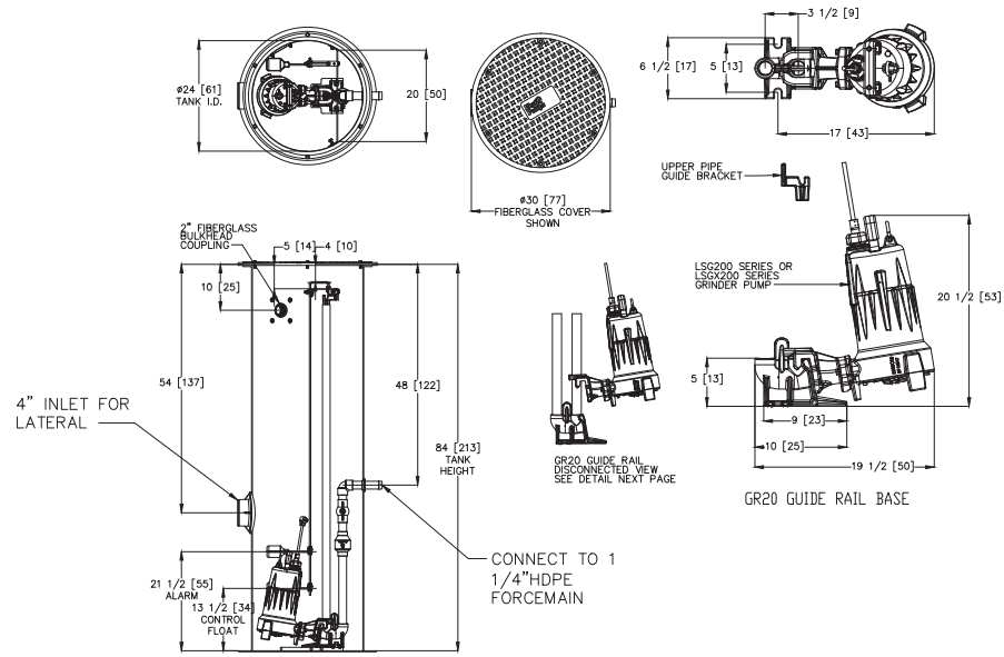
SIMPLEX GRINDER PUMP STATION SCALE: NTS
