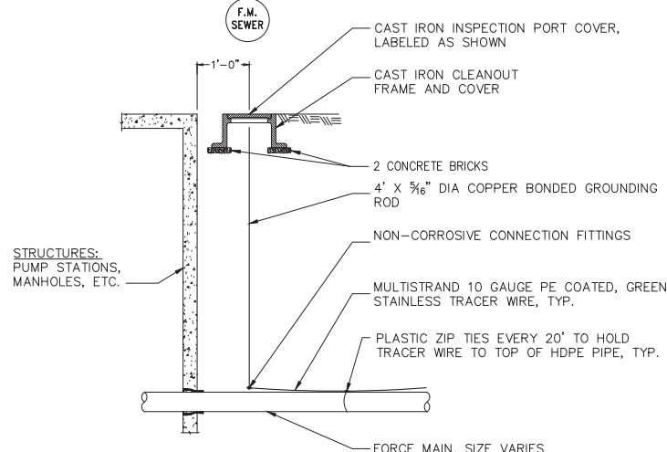
TYPICAL BEGINNING / END OF FORCEMAIN TRACER WIRE DETAIL SCALE: NTS
