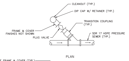
FORCEMAIN TO MANHOLE CLEANOUT
