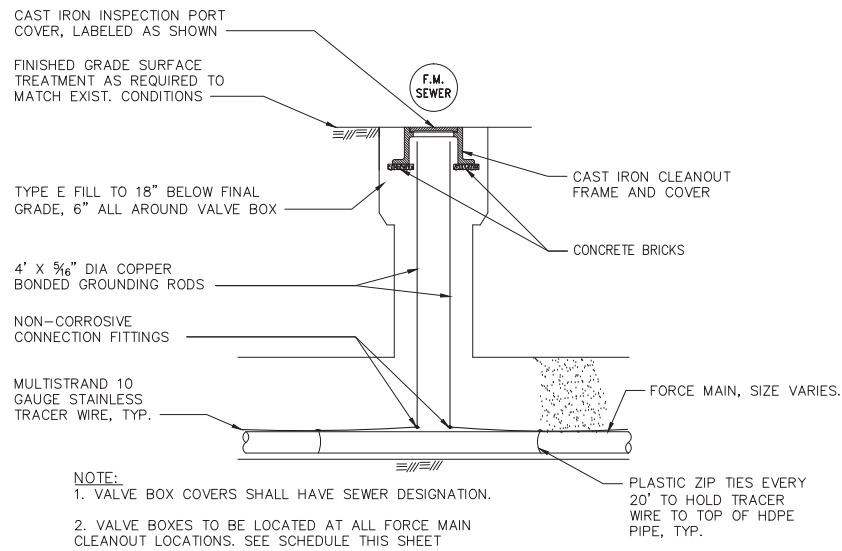
TYPICAL HDPE FORCE MAIN TRACER WIRE DETAIL SCALE: NTS
